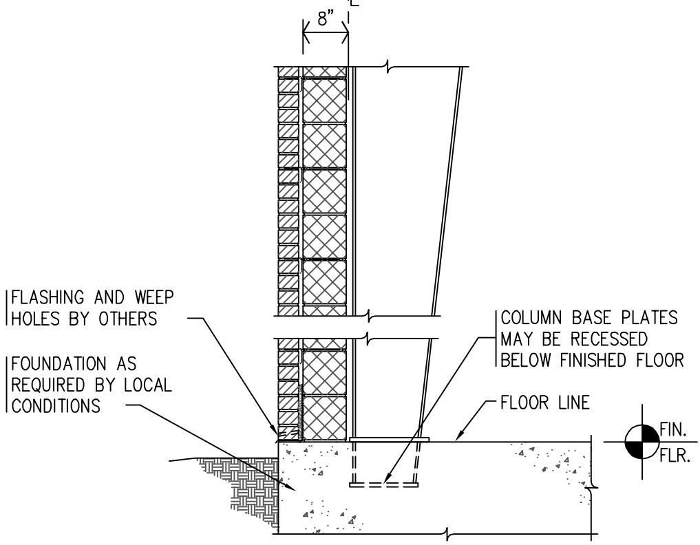
XX SECTION XX APPLICABLE TO ALL LANDMARK 2000 FRAMES SCALE: 1/2" = 1'-0"
