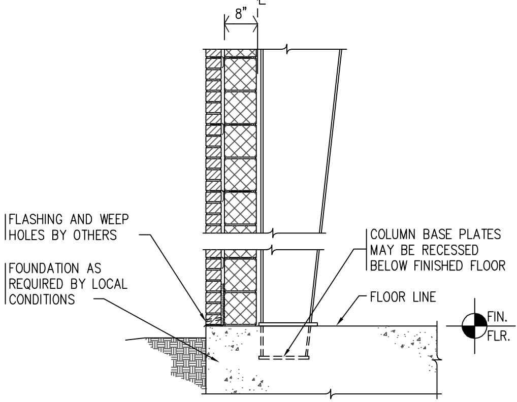
XX SECTION XX APPLICABLE TO ALL WIDESPAN FRAMES SCALE: 1/2" = 1'-0"
