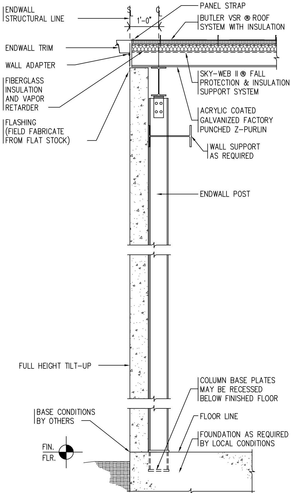
XX SECTION XX APPLICABLE TO ALL WIDESPAN FRAMES SCALE: 1/2" = 1'-0"
