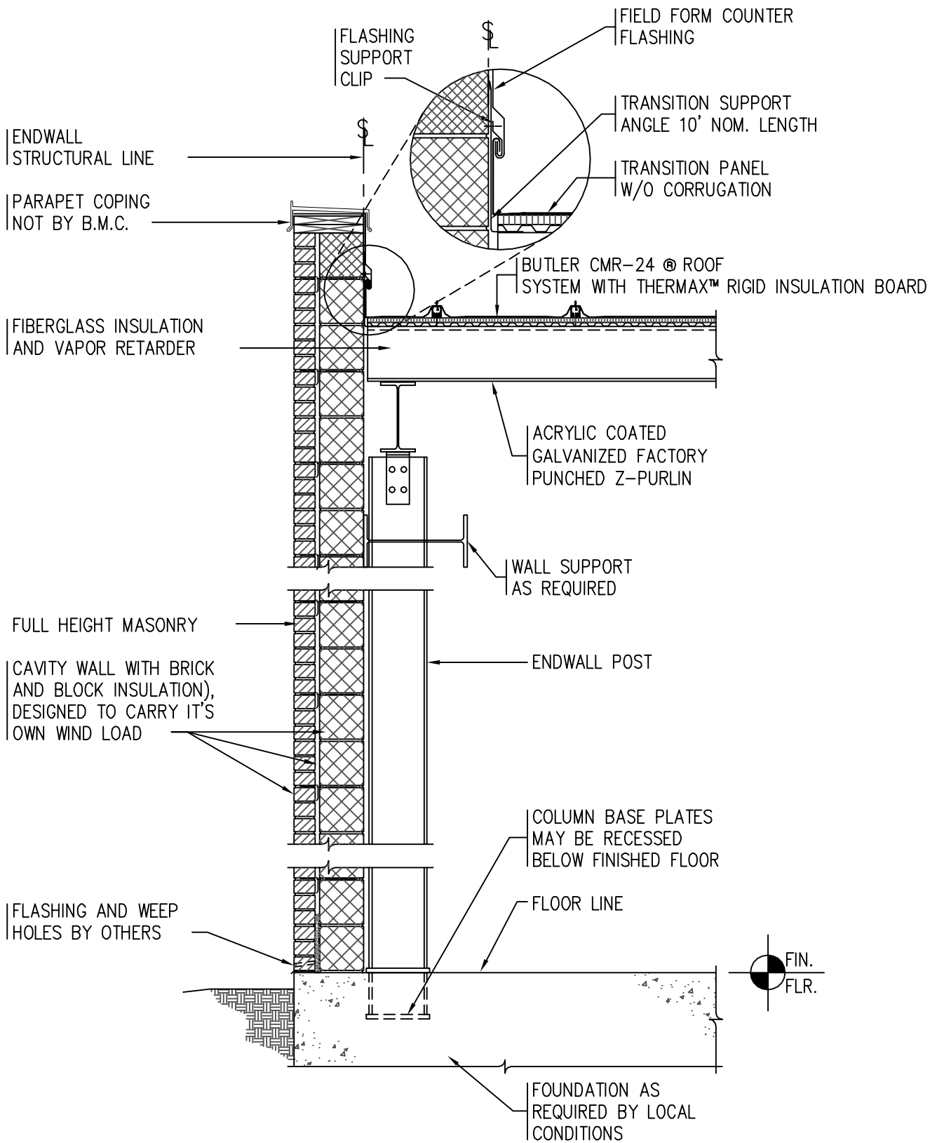
(XX) SECTION (XX) APPLICABLE TO ALL WIDESPAN FRAMES SCALE: 1/2" = 1'-0"
