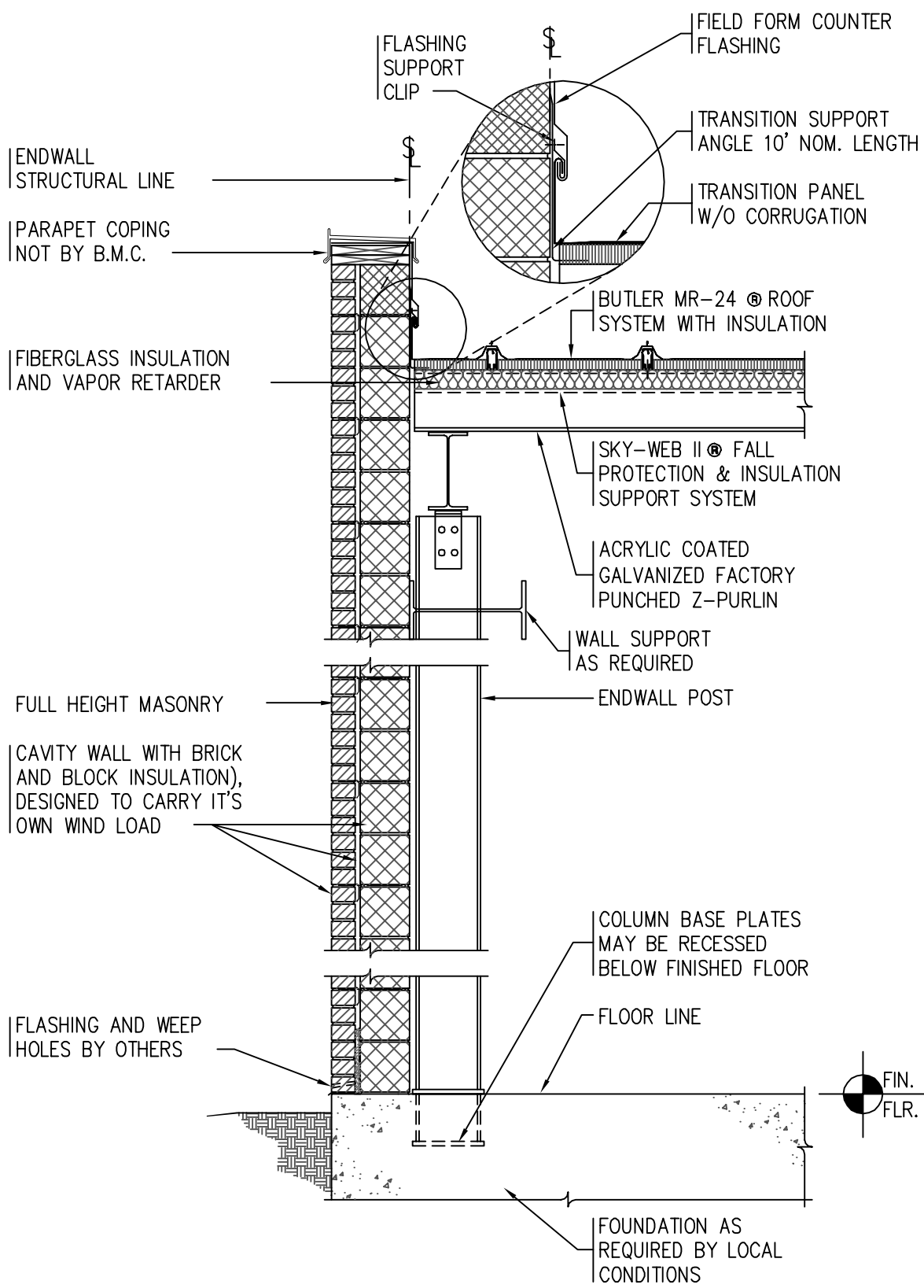
(XX) SECTION (XX) APPLICABLE TO ALL WIDESPAN FRAMES SCALE: 1/2" = 1'-0"
