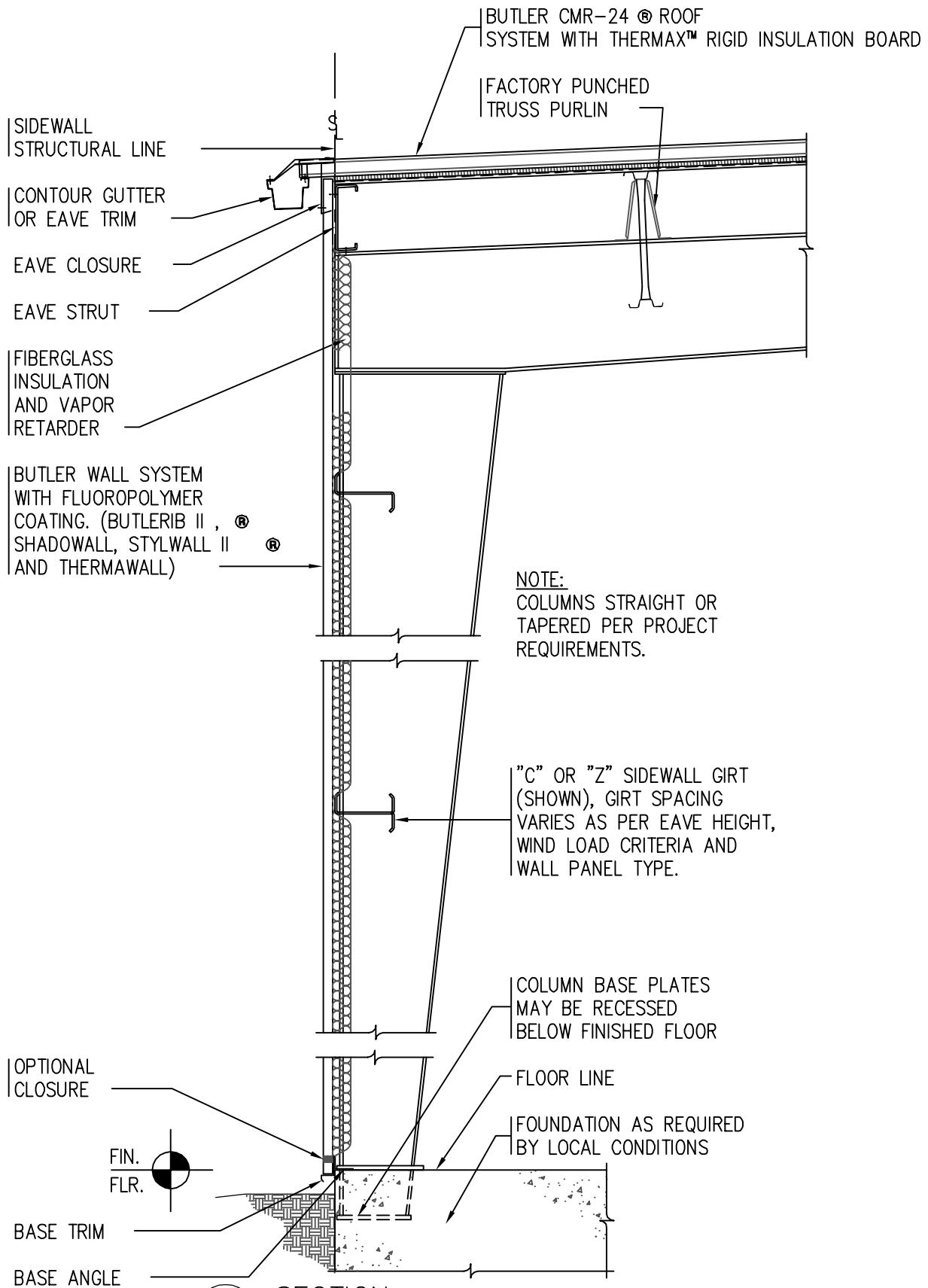
XX SECTION XX APPLICABLE TO ALL LANDMARK 2000 FRAMES SCALE: 1/2" = 1'-0"
