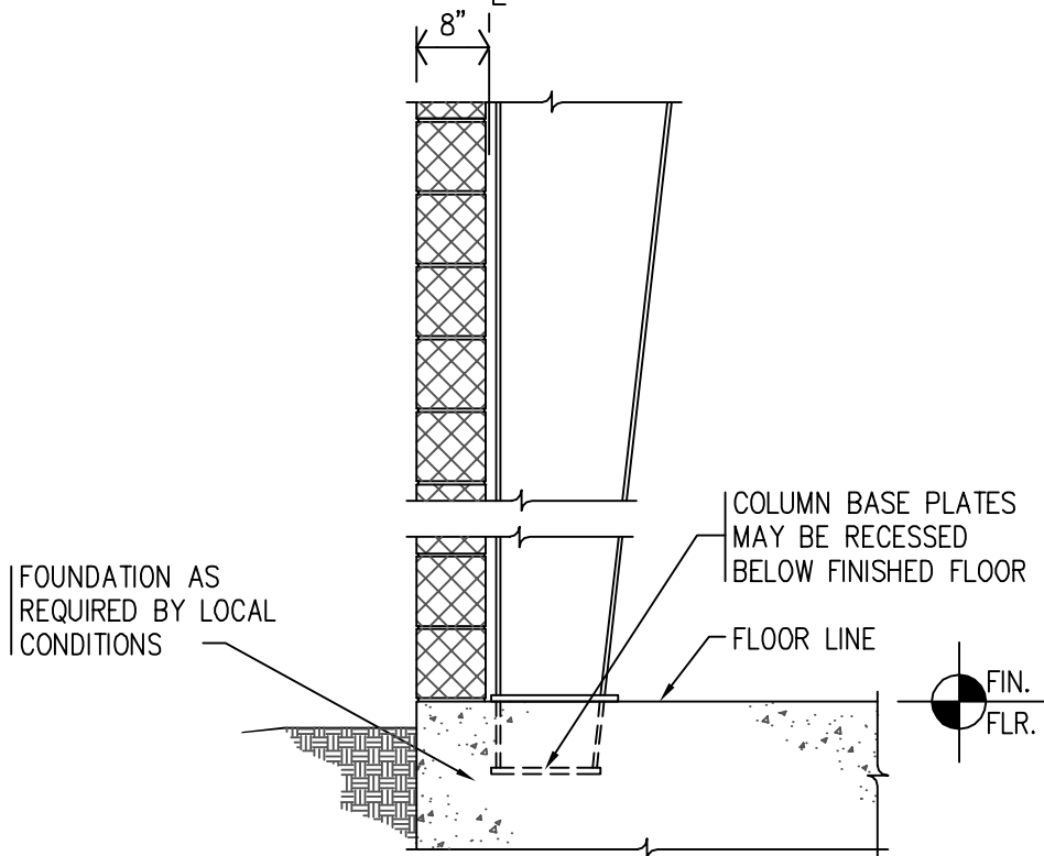
XX SECTION XX APPLICABLE TO ALL LANDMARK 2000 FRAMES SCALE: 1/2" = 1'-0"
