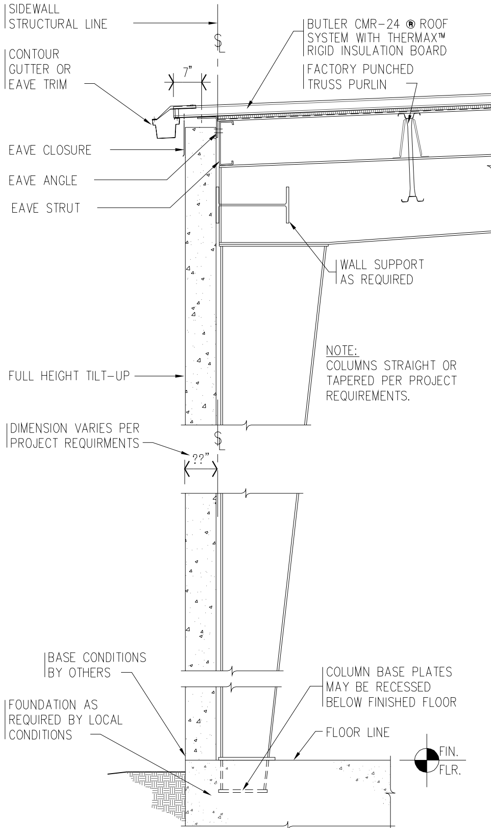
XX SECTION XX APPLICABLE TO ALL LANDMARK 2000 FRAMES SCALE: 1/2" = 1'-0"
