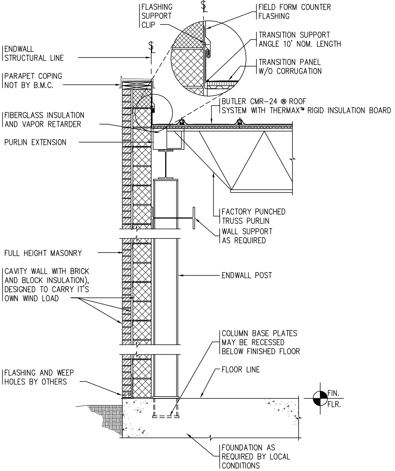
XX SECTION XX APPLICABLE TO ALL LANDMARK 2000 FRAMES SCALE: 1/2" = 1'-0"
