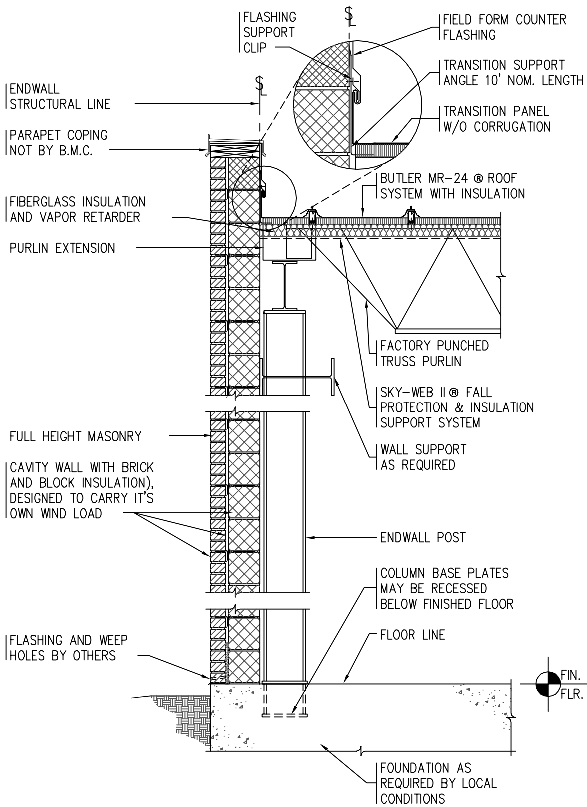
(XX) SECTION (XX) APPLICABLE TO ALL LANDMARK 2000 FRAMES SCALE: 1/2" = 1'-0"
