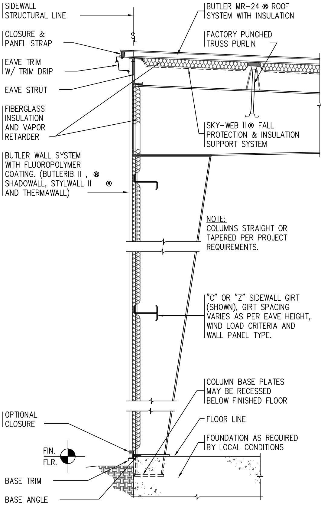
XX SECTION XX APPLICABLE TO ALL LANDMARK 2000 FRAMES SCALE: 1/2" = 1'-0"
