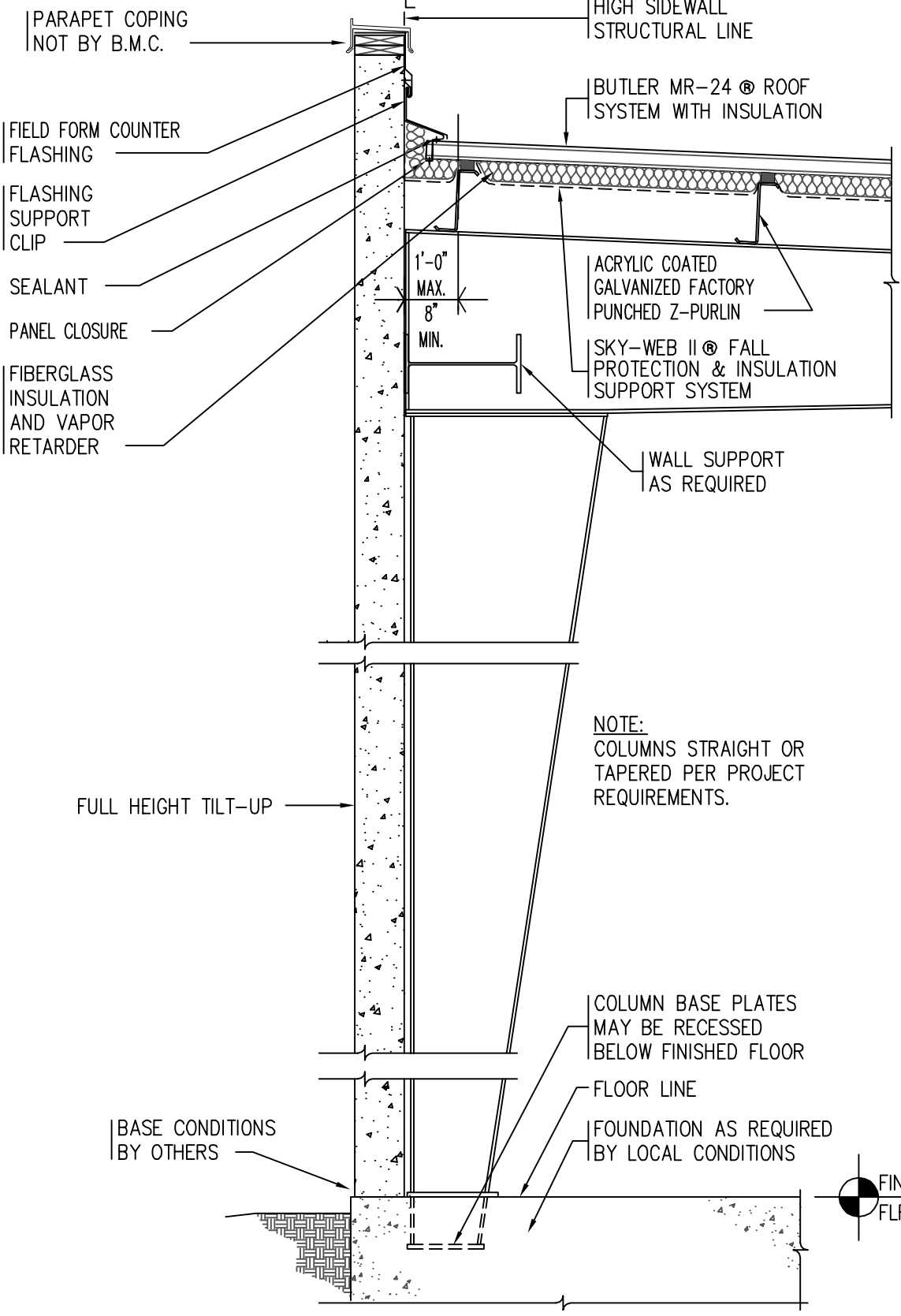
XX SECTION XX APPLICABLE TO ALL WIDESPAN FRAMES SCALE: 1/2" = 1'-0"
