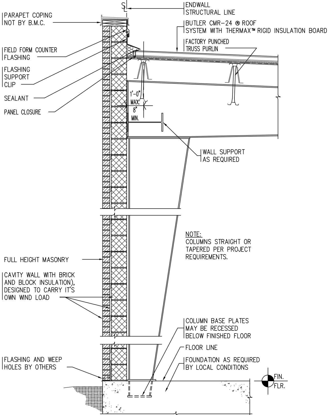
XX SECTION XX APPLICABLE TO ALL WIDESPAN FRAMES SCALE: 1/2" = 1'-0"
