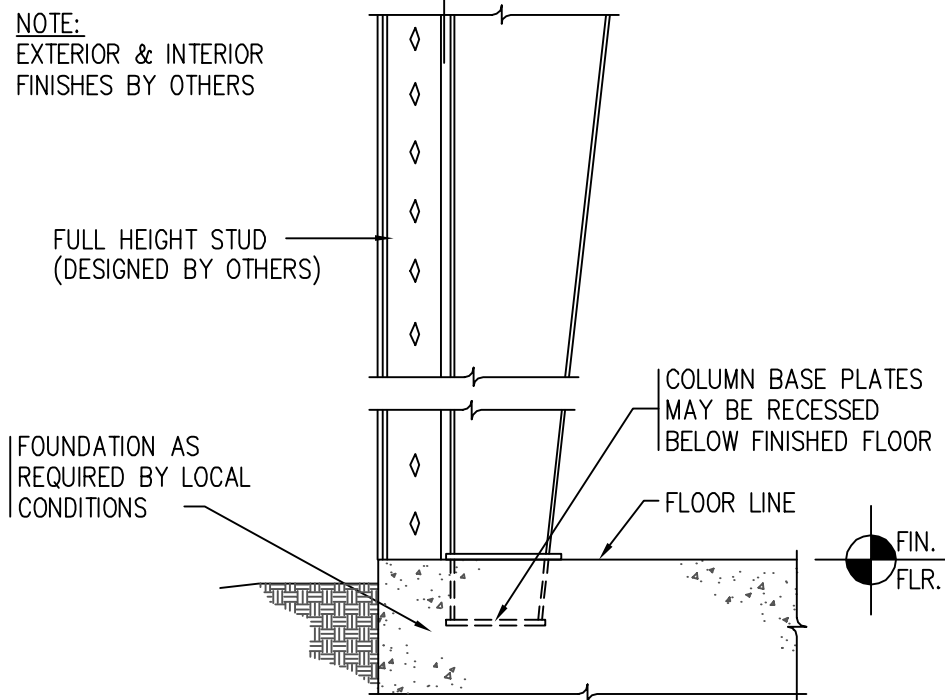
XX SECTION XX APPLICABLE TO ALL LANDMARK 2000 FRAMES SCALE: 1/2" = 1'-0"
